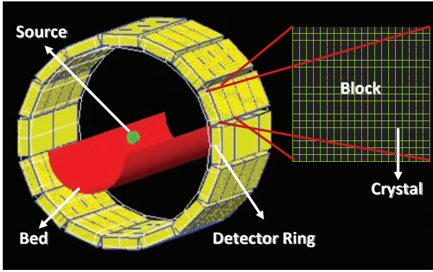
Fig. 1. Graphical representation of the geometry of the Inveon PET system as visualized by GATE. The LSO layer is depicted with yellow color.
