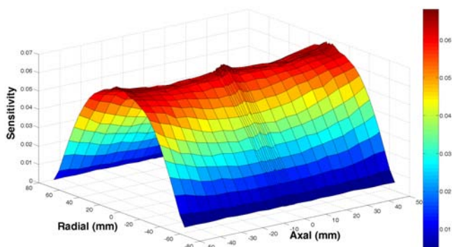
Fig. 2. Simulated sensitivity for complete FOV of the Inveon scanner.
