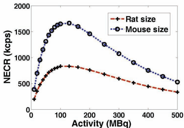
Fig. 3. Plots of simulated NECR as a function of total activity for mouse- and rat-sized phantoms.
